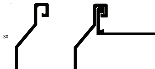
Assembled
